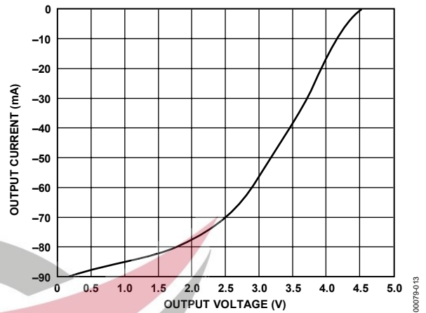
Figure 18. Output Current vs. Driver Output High Voltage
